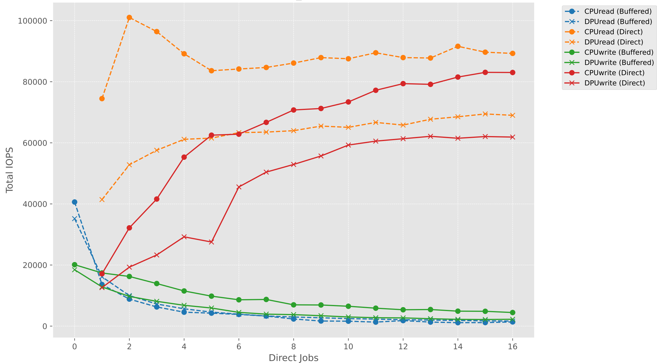
IOPS vs Direct Jobs (buffered1_directN) - SEQ (CPU vs DPU)
